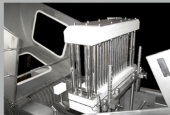
Stainless Steel 4 mm needles
