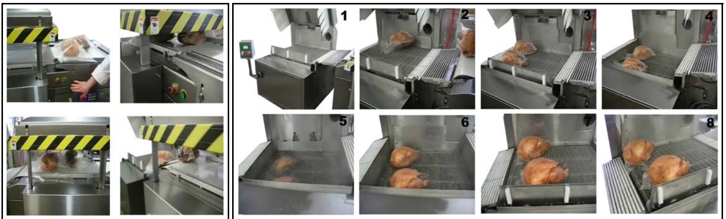
Belted Vacuum Packaging Machine
